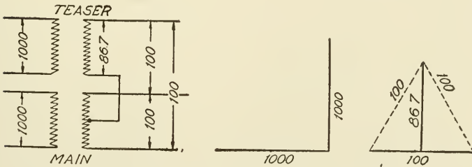
Fig. 32. Diagram of Scott Connections and Vector Diagrams for Same
